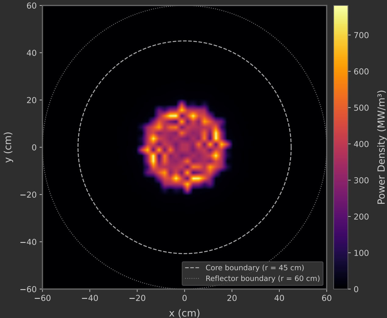
AYURI Core — Reconstructed Full-Core Radial Power (from 1/12 symmetry, at z = 0 )
